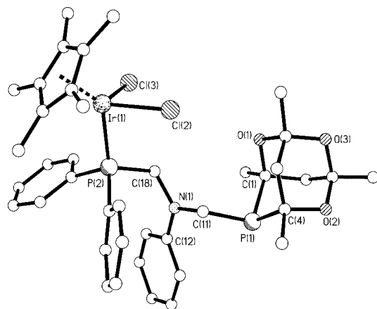
Figure 7. Molecular structure of 7 ; all hydrogen atoms and solvent have been removed for clarity.
