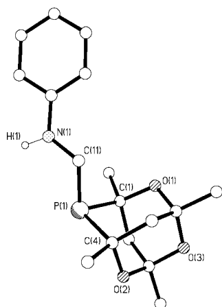
Figure 2. Molecular structure of 2a ; all hydrogen atoms except on \text{N}(1) have been removed for clarity.
