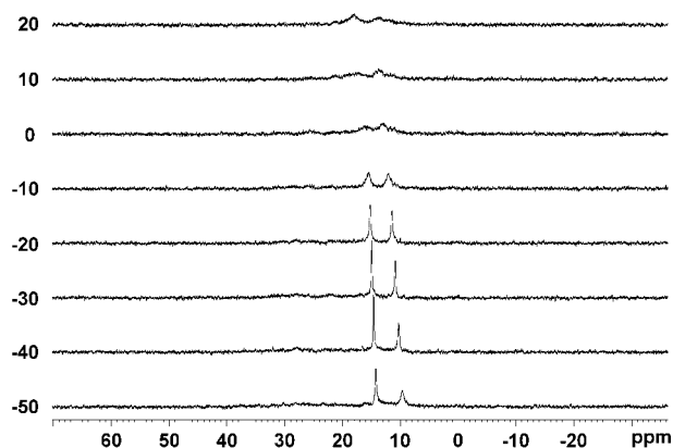
Figure 10. Variable temperature ^{31}\text{P}\{^1\text{H}\} NMR spectra for 10 recorded in the range 20 to -50^\circ\text{C} .
