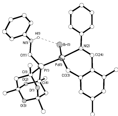
Figure 3. Molecular structure of 4 . All hydrogen atoms except on N(1) have been removed for clarity.
