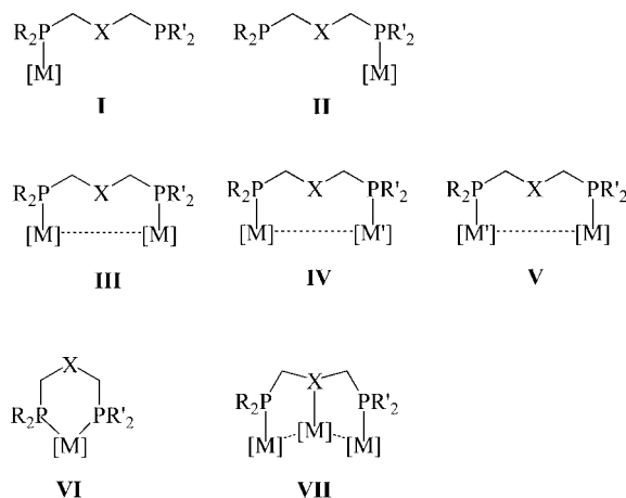
Figure 1. Schematic representation of the possible coordination modes for R 2 PCH 2 XCH 2 PR' 2 .
