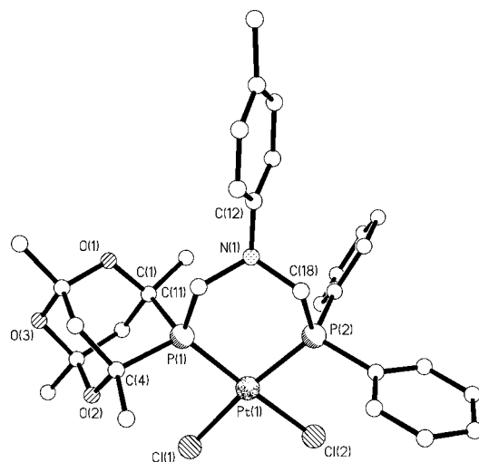
Figure 5. Molecular structure of 5b . All hydrogen atoms and solvent have been removed for clarity.
