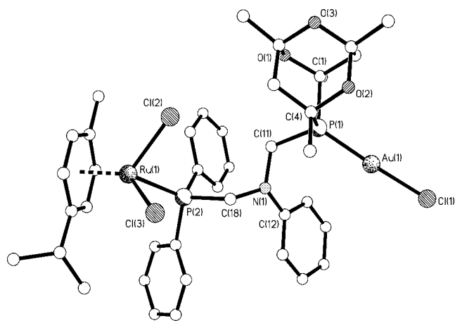
Figure 8. Molecular structure of 8 ; all hydrogen atoms and solvent have been removed for clarity.
