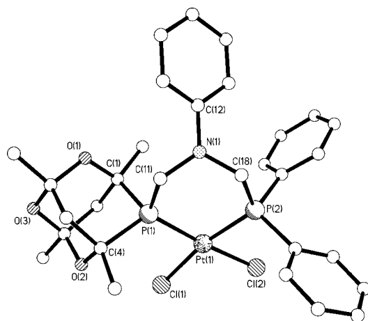
Figure 4. Molecular structure of 5a . All hydrogen atoms and solvent have been removed for clarity.
