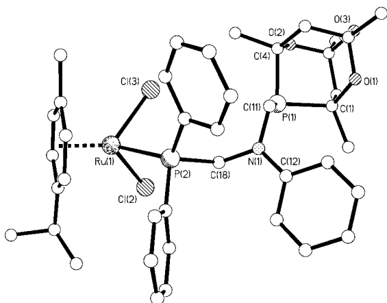
Figure 6. Molecular structure of 6 ; all hydrogen atoms and solvent have been removed for clarity.
