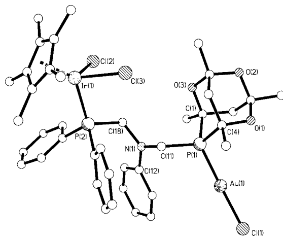
Figure 9. Molecular structure of 9 ; all hydrogen atoms have been removed for clarity.
